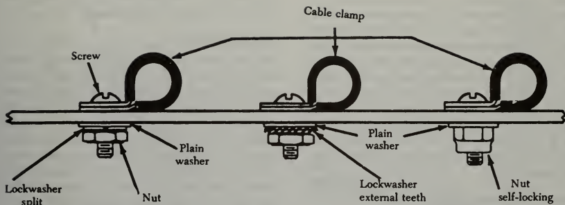
FIGURE 4-97. Typical mounting hardware for cable clamps.
